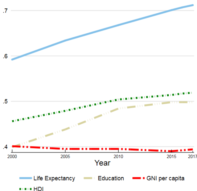
Figure 1: Trends in Madagascar's HDI component indices 2000-2017
