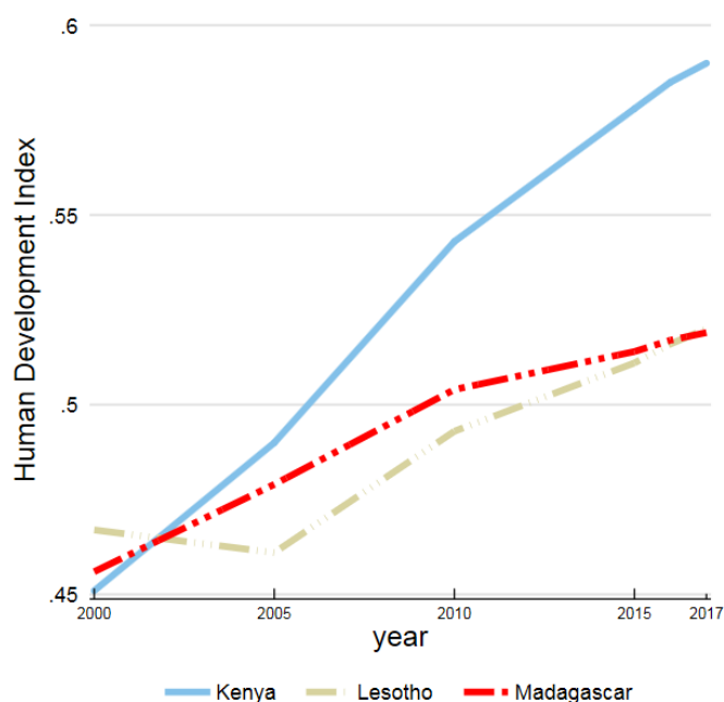
Figure 2: HDI trends for Madagascar, Kenya and Lesotho, 2000-2017
